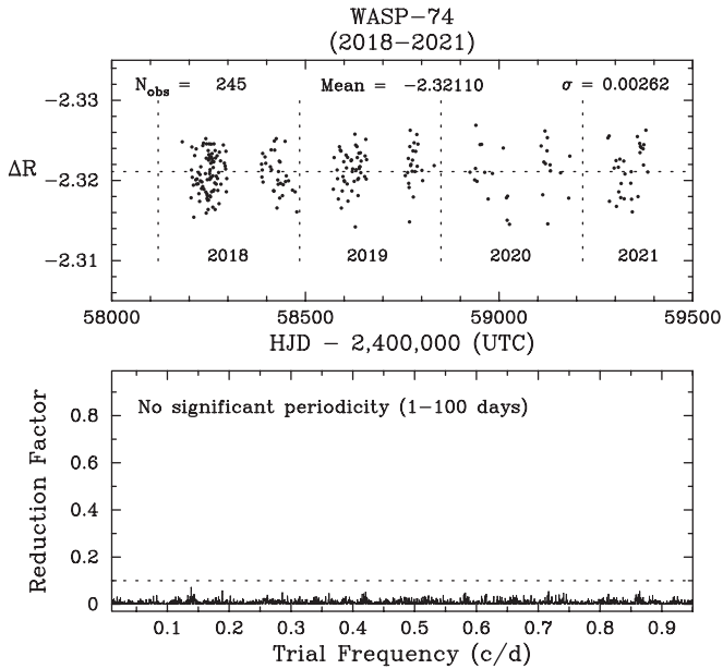
Figure 4. Top: the Cousins R -band photometry of WASP-74 from 2018–2021, acquired with the C14 AIT at Fairborn Observatory. The star is constant on night-to-night and year-to-year timescales to the limit of our precision. Bottom: frequency spectrum of the complete data set shows no significant periodicity between 1 and 100 days. The horizontal dashed line in the bottom panel represents the noise limit below which reliable periods are not found in multicolor photometry (Henry et al. 2011).
