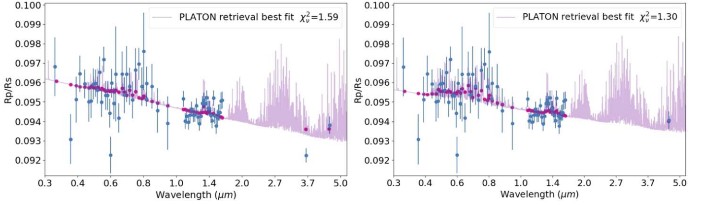
Figure 7. Best-fit PLATON retrieval of WASP-74b transit spectrum. The purple line is the full-resolution model with pink dots for corresponding binned model. The left panel uses the full spectrum and the right panel excludes the 3.6 \mu\text{m} point. We see strong scattering with muted water feature and no evidence for TiO absorption or super-Rayleigh scattering in both retrievals. However, the low 3.6 \mu\text{m} point does drive up the cloud scattering factor.
