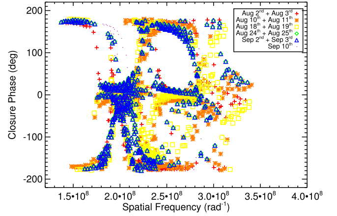
Figure 9. Observed closure phases for the 2010 data set. The errors bars, excluded for clarity, range between 1^\circ 02' and 114^\circ with a median error of 3^\circ 24' . The distinct nonzero closure phase signature points to surface asymmetries. The differences in the closure phase between nights indicates an evolving asymmetric surface pattern from night to night.
