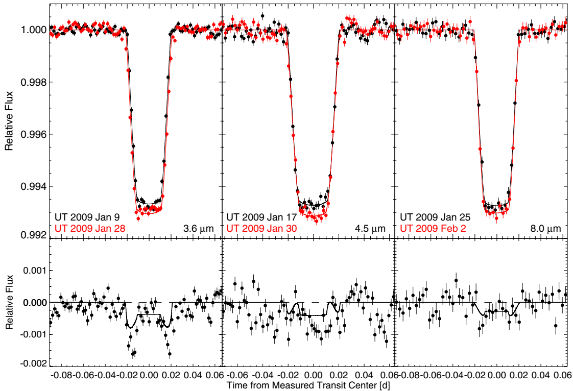
Figure 13. This plot shows the six transits observed in 2009 January/February. The left panel shows both 3.6\ \mu\text{m} transits, the middle panel shows both 4.5\ \mu\text{m} transits, and the right panel shows both 8.0\ \mu\text{m} transits. The upper part of each panel overplots the normalized photometry for each visit (filled circles), with the first visit in black and the second visit in red, along with the best-fit transit light curves (solid lines) where the orbital inclination, a/R_* , and transit time have been allowed to vary freely for each individual transit. The lower panel takes the difference between the two light curves (black filled circles) and compares it to the difference between the best-fit transit solutions (solid black line). Note that even when all transit parameters are allowed to vary freely, it is not possible to reproduce the sharp features visible during ingress and egress in the lower left panel.
