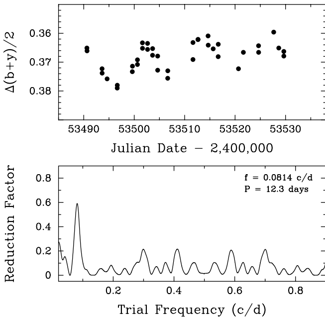
FIG. 9.— Top : Strömgren (b+y)/2 photometric observations of HD 102195 obtained at the end of the 2004–2005 observing season with the T10 0.8 m APT at Fairborn Observatory. A cyclic variation of about 0.015 mag in the brightness of the star is easily seen. Bottom : Power spectrum of the observations in the top panel. A clear period of 12.3 days is interpreted as the rotation period of the star.
