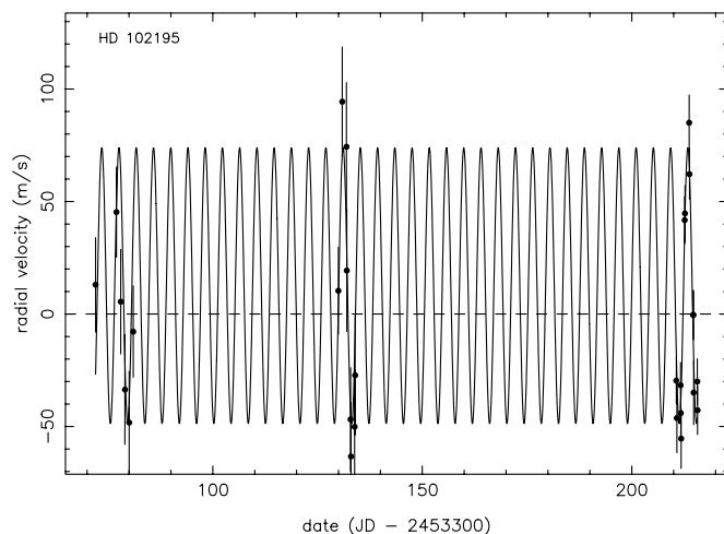
FIG. 2.—Radial velocities for HD 102195, showing the 28 measurements from ET at the KPNO coude feed/2.1 m in the spring of 2005. The rms errors for the ET measurements at KPNO are \sim 10 and \sim 20 \text{ m s}^{-1} for the 2.1 m and coude feed, respectively. The solid line is the Keplerian orbital fit to the observed data.
