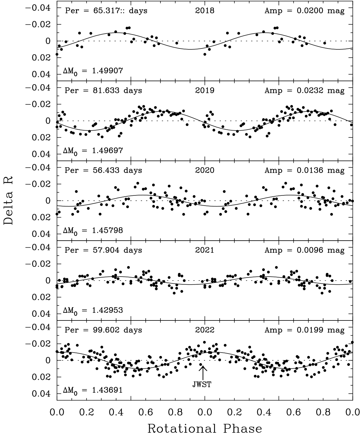
Figure 2. Cousins R band phase curves of GJ 1214 from 2018 to 2022. Periods for each year are given in the upper left of each panel. Peak-to-peak amplitudes are given in the upper right. Like the results given in the literature, our periods cover a broad range. The arrow in the bottom panel marks the phase of the July 20-22, 2022 JWST observation.
