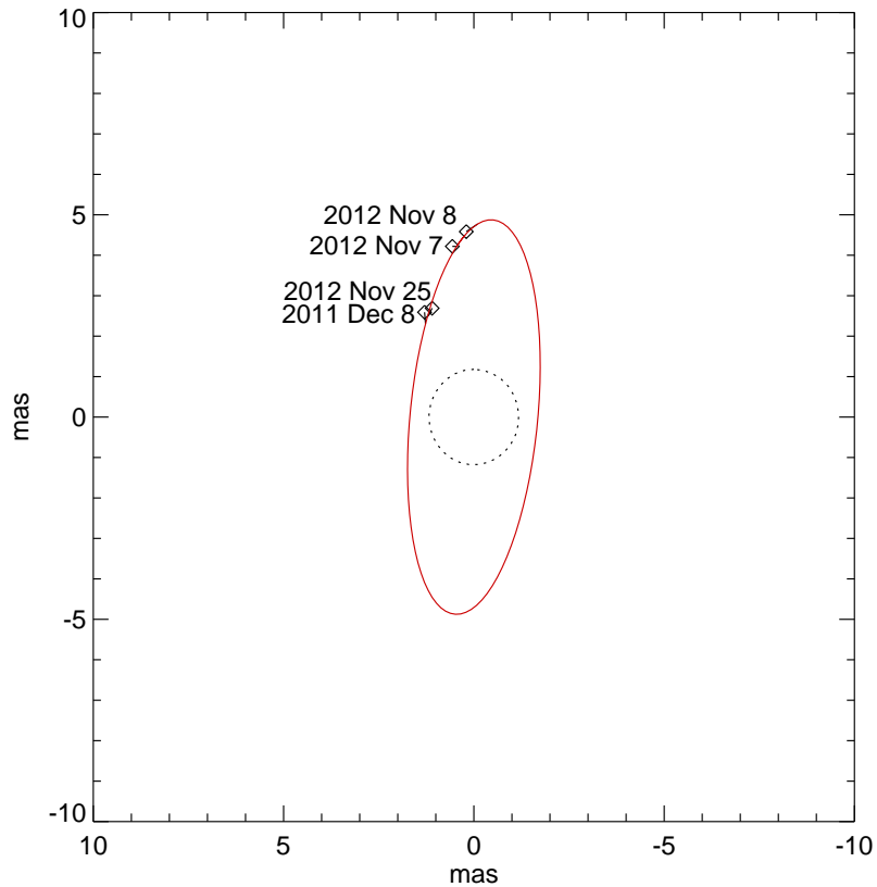
Figure .2: Visual orbit of \sigma Geminorum. The black diamonds indicate our four interferometric detections of the secondary star. The red ellipse is our orbit fit. The dotted ellipse is the outline of the primary star (Roettenbacher et al. in prep.).
