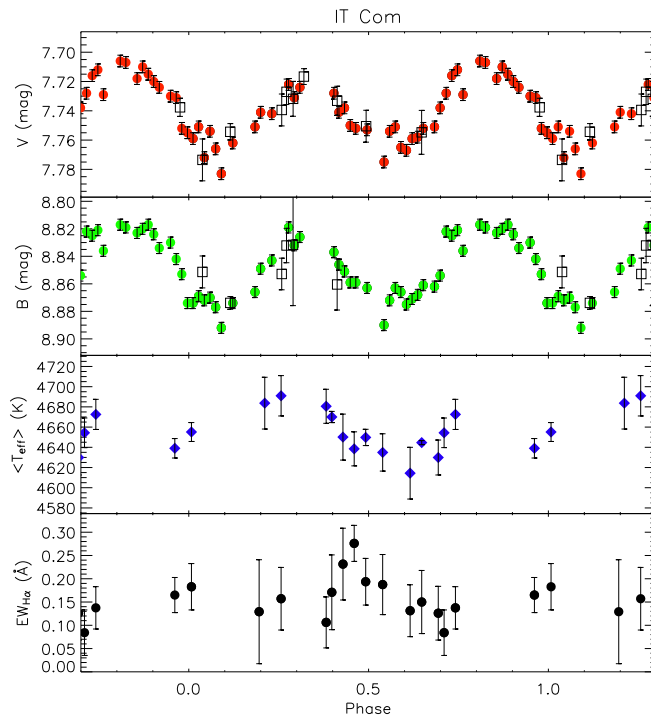
Figure 1. From top to bottom. V and B magnitudes, averaged T_{\text{eff}} and EW_{\text{H}\alpha} as a function of rotational phase. In the light curves, the filled circles are FO data, while the empty squares are \text{COM}\ddot{\text{U}} photometry. For the photometric observations, HD 117816 ( V = 8^{\text{m}}48 , B = 10^{\text{m}}05 ) was used as comparison star, while HD 119126 ( V = 5^{\text{m}}58 , B = 6^{\text{m}}59 ) was chosen as check star (Yoss & Griffin, 1997). A shift has been applied to the few \text{COM}\ddot{\text{U}} data in order to adequately match those ones from FO
