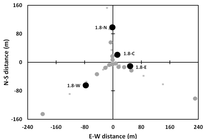
Fig. 3. Planned locations of the 1.8m telescopes (filled black circles). Filled gray circles indicate the stations already available plus the new stations shown in Fig. 2. As in Figs. 1 and 2, the small gray squares are station locations not yet in use.
