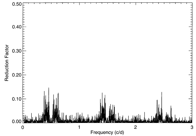
Figure 2. A power spectrum of the complete B -band photometric data set after removal of the \nu = 0.385\,53\,d^{-1} signal.
