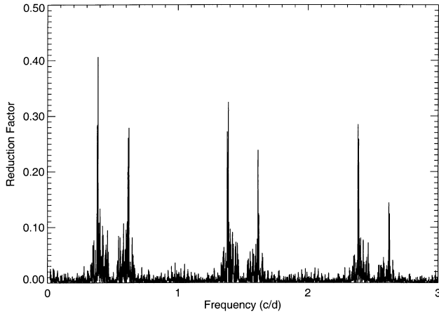
Figure 1. A power spectrum of the complete B -band photometric data set showing a single frequency ( \nu = 0.385\,53\,d^{-1} ) and its one cycle per day aliases.
