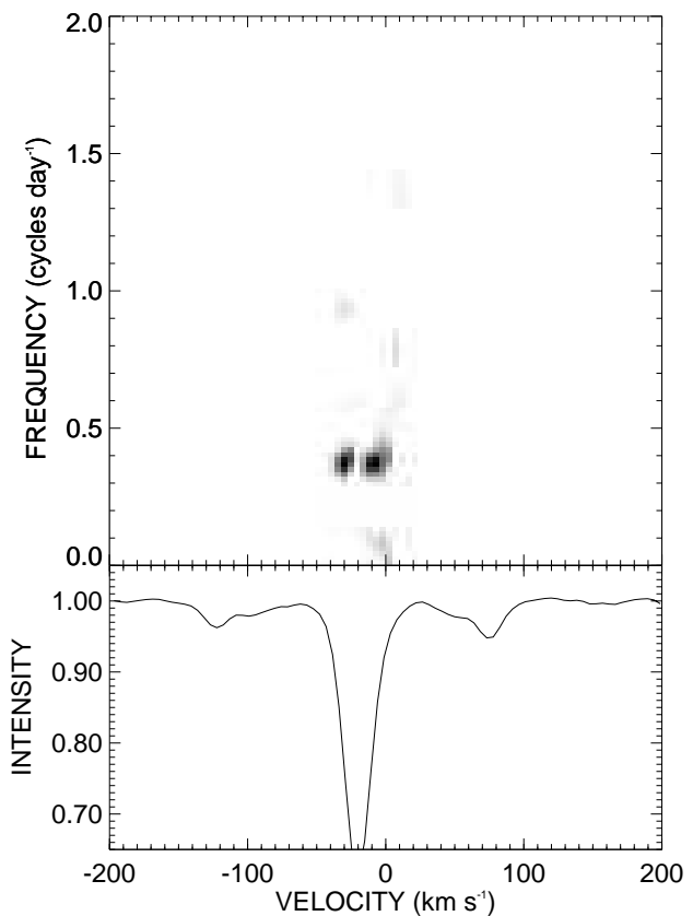
Figure 4. Periodogram for HR 8330 across the Fe II \lambda 4508.289 line. Note the distribution of power across the line profile.
