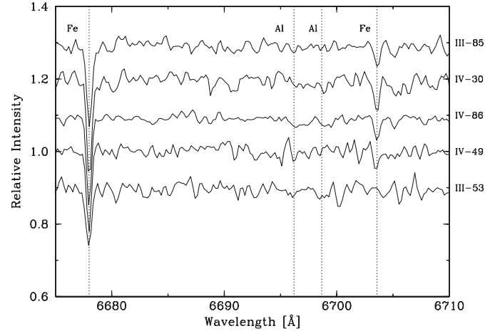
FIG. 1.—Spectra from all five program stars are shown with a pair of Fe I and Al I lines indicated for reference. The spectra have been offset for display purposes.
