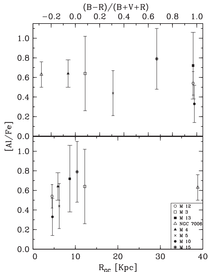
FIG. 3.—Top panel shows [Al/Fe] vs. the horizontal-branch parameter, where a value of +1.0 means only BHB stars, 0.0 is a mix of RHB, BHB, and RR Lyrae stars, and -1.0 means only RHB stars. The various symbols indicate the average [Al/Fe] abundance in a cluster with the error bars showing the 1\sigma values. The bottom panel shows [Al/Fe] vs. the Galactocentric distance for each cluster. The cluster data are from the following sources: M12 (Johnson & Pilachowski 2006), M3 and M13 (Johnson et al. 2005), NGC 7006 (Kraft et al. 1998), M4 (Ivans et al. 1999), M5 (Ivans et al. 2001), and M15 (Snedden et al. 1997).
