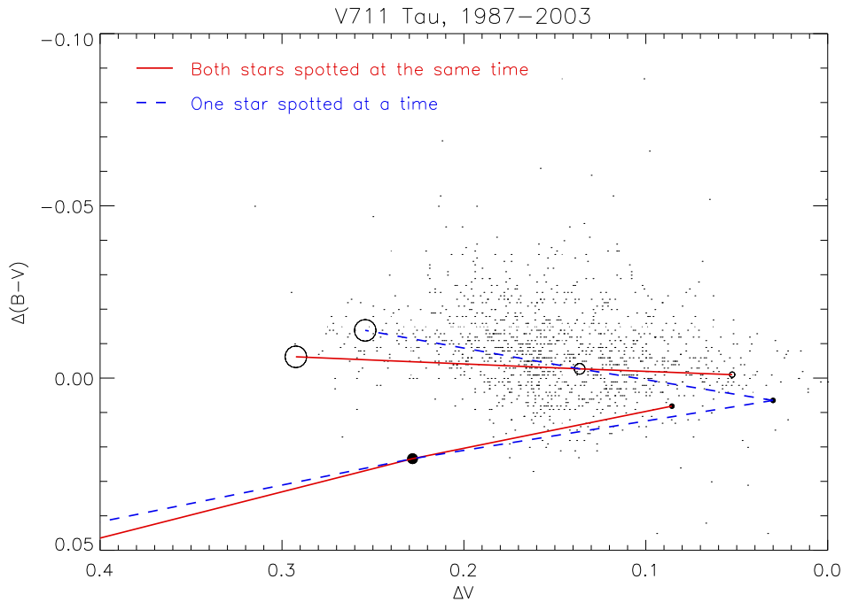
Figure 1. Theoretical calculations of \Delta V and \Delta(B - V) of the V711 Tau system relative to the V711 Tau system where Aa and Ab are both unspotted. The observations are shown as dots. The filled circles represent models where the active regions contain only dark spots. The open circles represent models where the Aa active regions also contain faculae.
